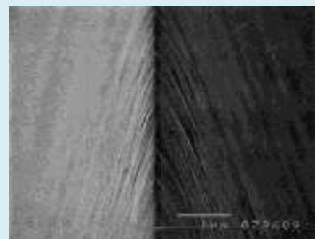
Observation on blade edge (SEM x 20,000)
